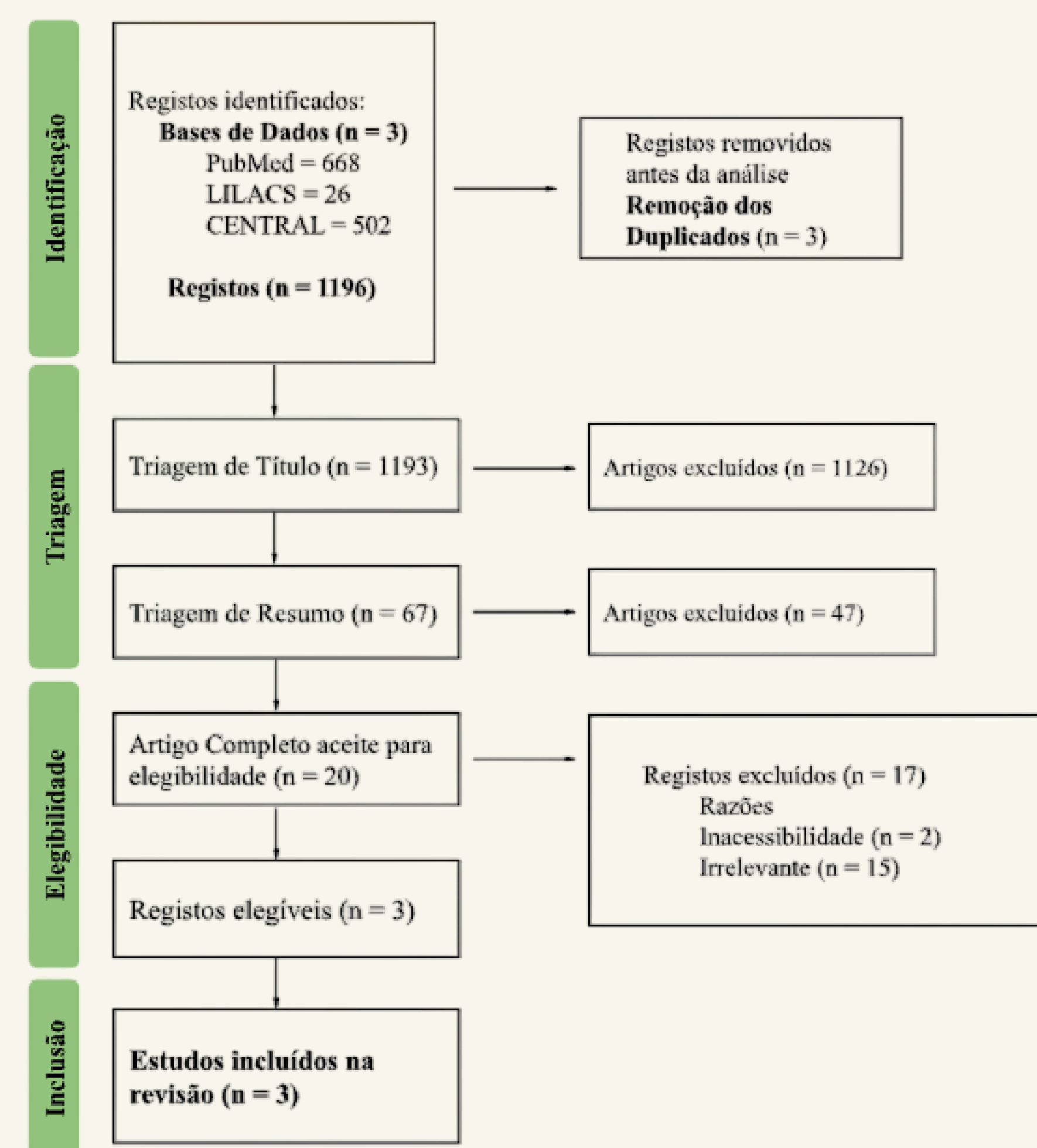
Figura 1 - Prisma 2020 Flow Diagram (Page et al., 2021)
